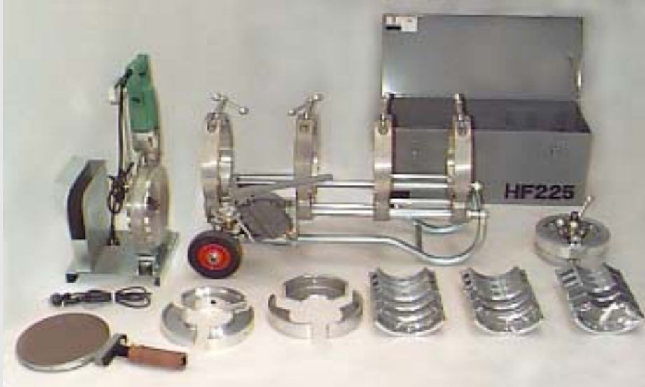
butt welding kit for pipe and fittings - 225mm to 63mm
