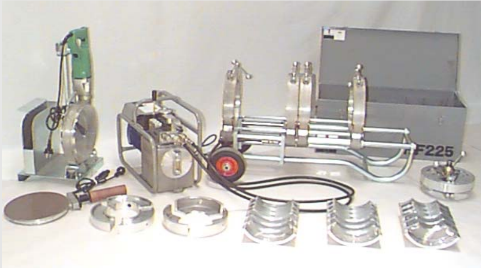
butt welding kit for pipe and fittings - 225mm to 63mm
